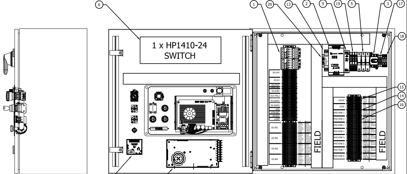
PANEL INTERNAL LAYOUT VIEW
