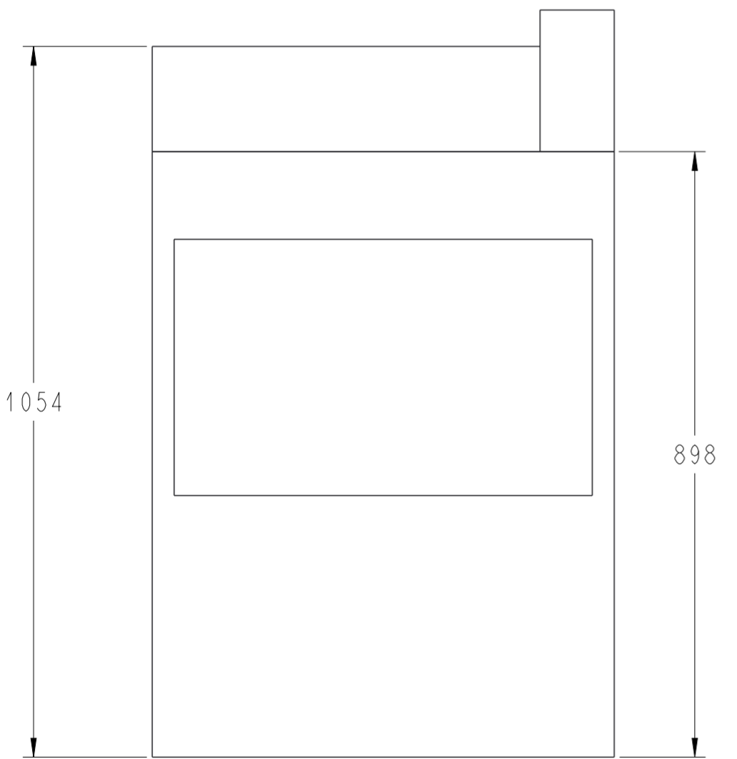
FRONT VIEW
