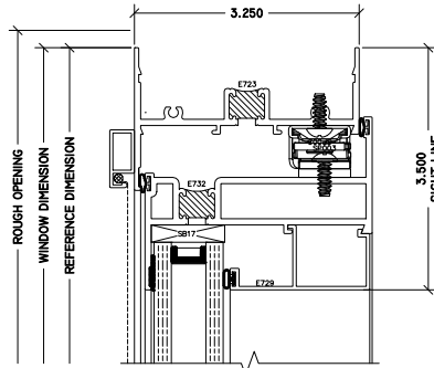
1 INSWING CSMT HEAD 320 CASEMENT
