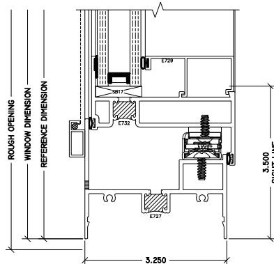
2 INSWING CSMT SILL 320 CASEMENT
