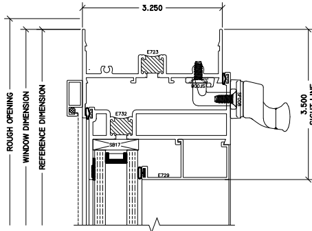
1 PI HEAD 320 PI
