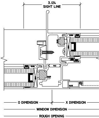
7 OX MTG RAIL 3210 HS
