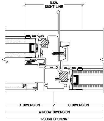
6 XO MTG RAIL 3210 HS
