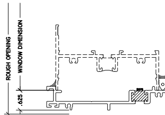
2 SUB SILL
