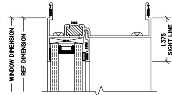
8 STACK HEAD 3250 FXD
