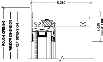
1 FX HEAD 3250 FXD
