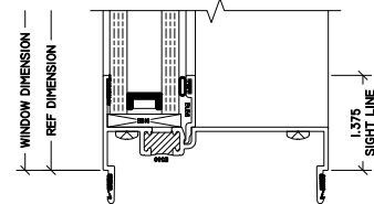
9 STACK SILL 3250 FXD
