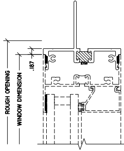
3 HEAD NAIL FIN
