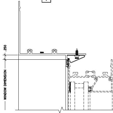
1 SQ. PANNING HEAD
