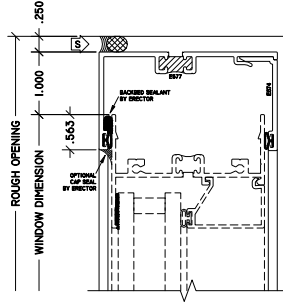
3 HEAD SUBFRAME
