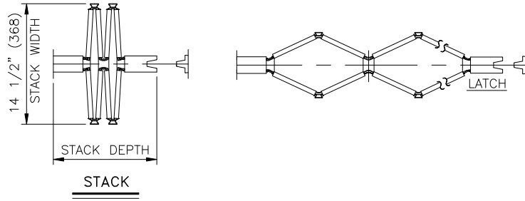
Single Fixed (Left Hand)-Jamb Partition
