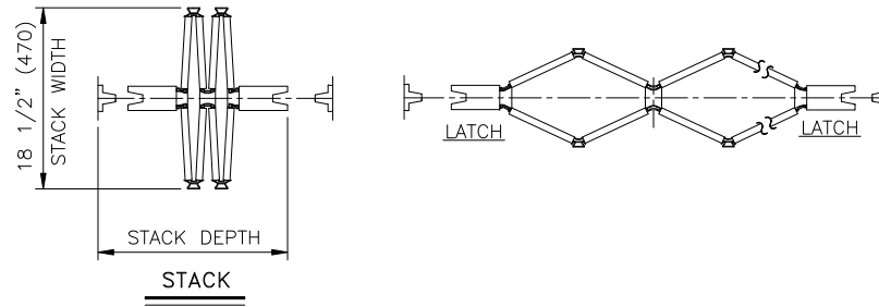
Double-End Post Partition
