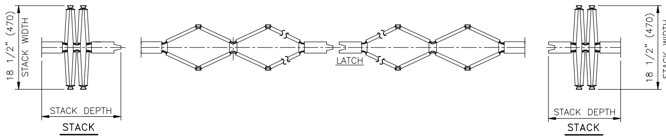
Joining Pair Of Fixed-Jamb Partitions
