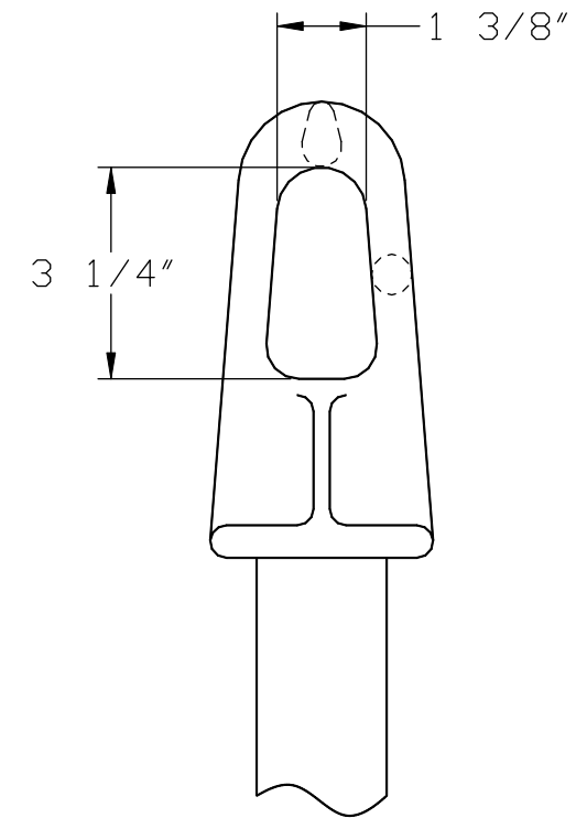
GALVANIZED STRAP EYE
