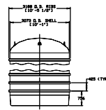
10' DIA AST-V
