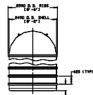
8' DIA AST-V
