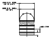
6' DIA AST-V
