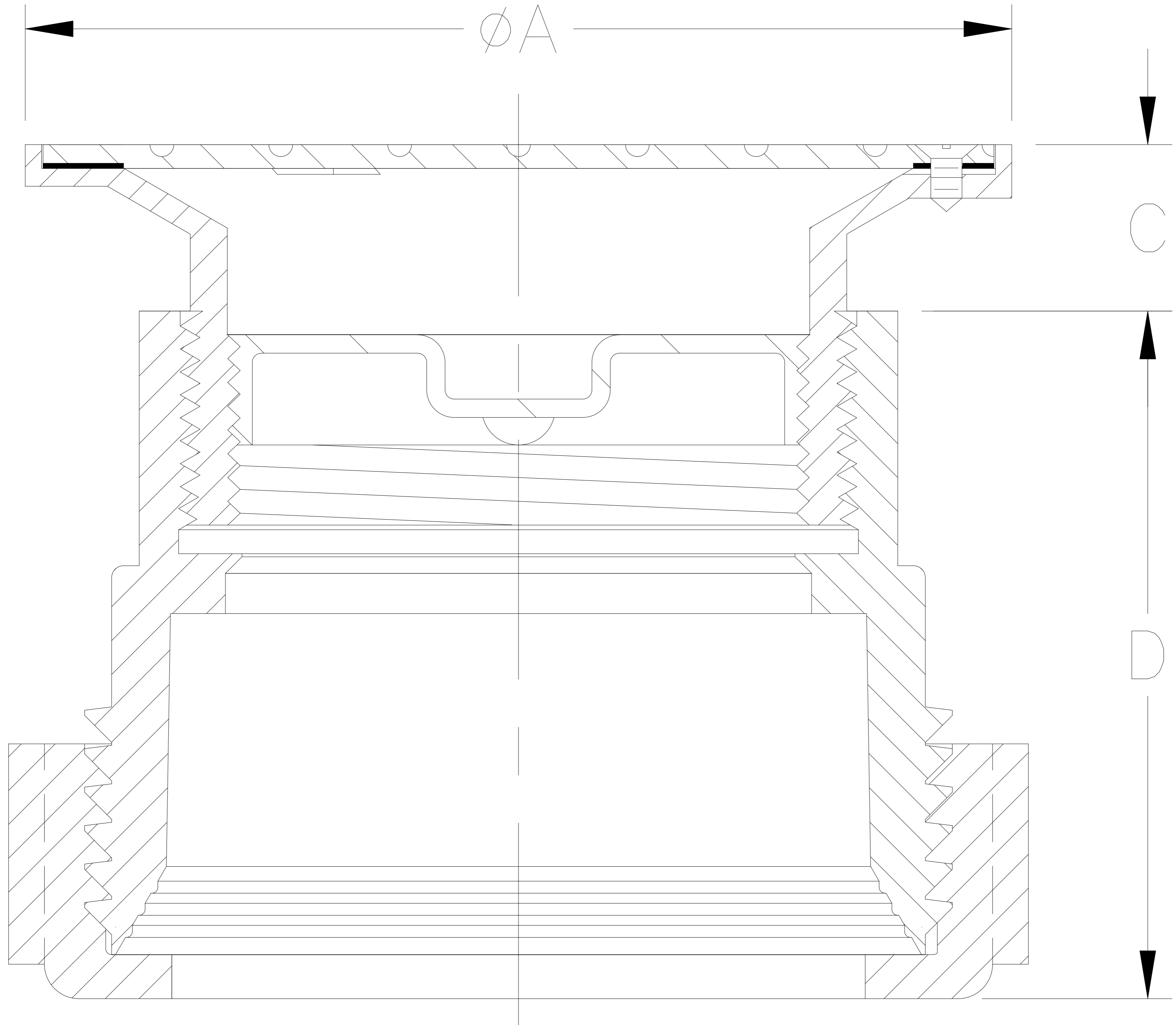
ZURN JOINT
