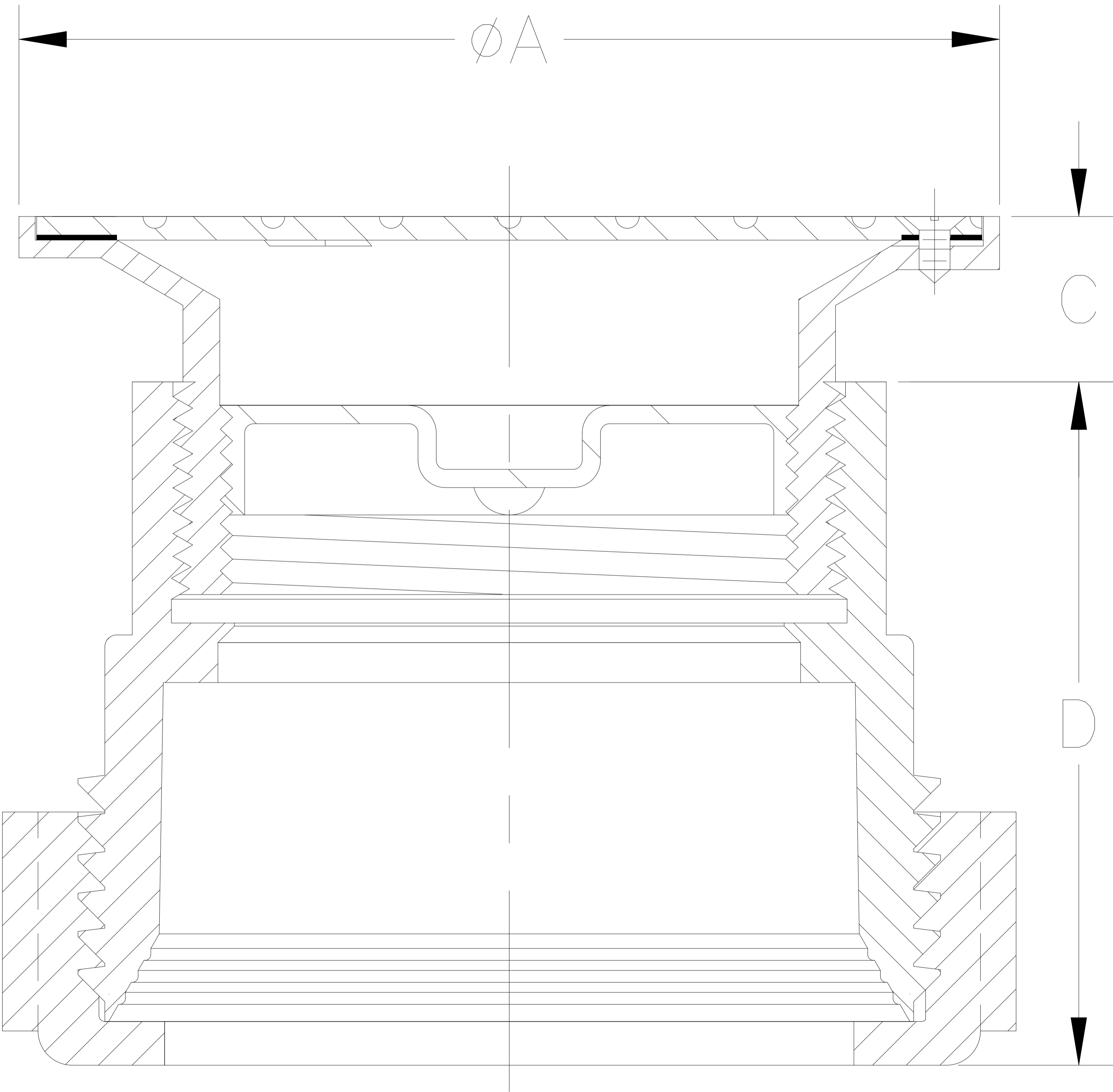
ZURN JOINT
