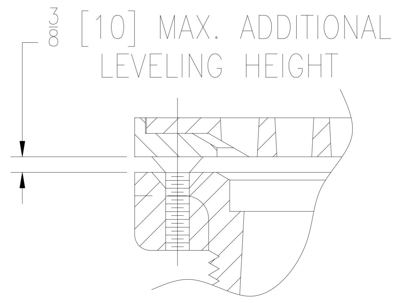
SECTION B-B
