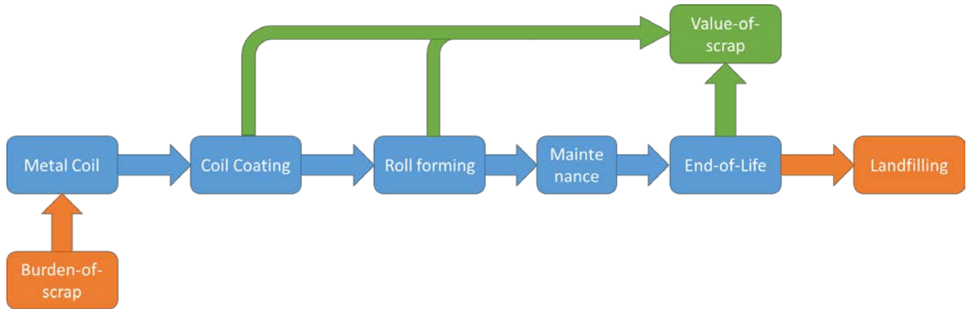
Figure 5: Cradle-to-grave system boundaries of roll-formed metal cladding
