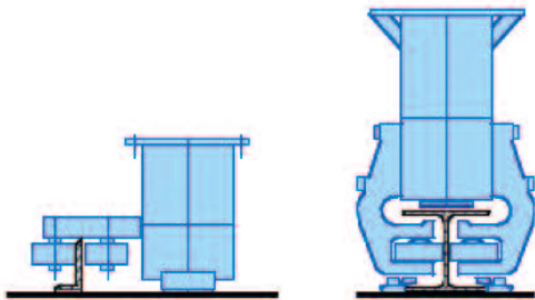
Fig 5 - Traversing on rails track, with 'L' shaped guide rail
