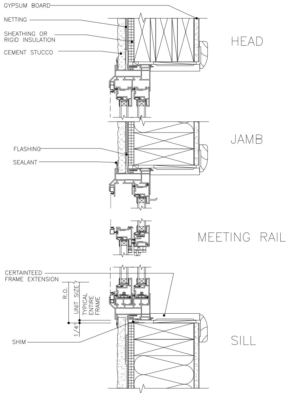
NEW CASTLE XT 2 LITE GLIDER STUCCO – 2x6 FRAME
