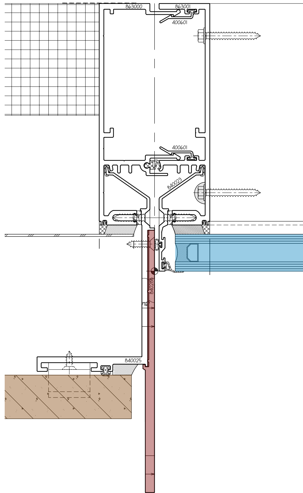
2 - VERTICAL DETAIL AT TERRACOTTA / VISION PM403 - SCALE: FULL
